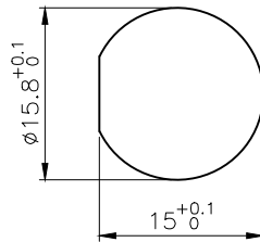
Dimensions of panel openings
